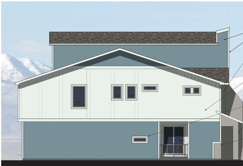
2 Typical Side Elevation - Courtyard Interior Location
